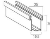
Guida in alluminio A30 GUIAL...30M 19,5 x 30 mm
