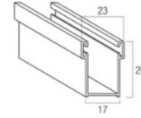
Guida in alluminio A28 GUIAL...28M 17 x 28 mm
