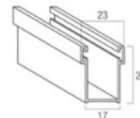
Guida in alluminio A28 GUAL...28M 17 x 28 mm
